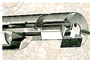
Twin Extractors and Recessed Bolt Face
